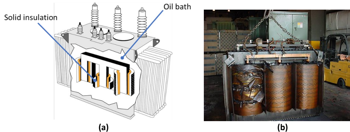
Figure. 1 Oil-immersed, 3-phase core-type power transformer: (a) Schematic highlighting the insulating elements, (b) picture showing degraded solid insulation inside a transformer. 99,100
