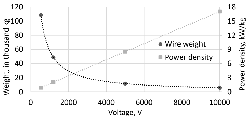
Fig. 1. Voltage vs. copper wiring weight (no insulation) 181 and power density.
