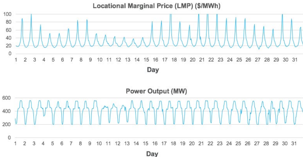
Figure 1: Day-ahead LMP 60 and the power output 61 of the Wolf Hollow II Generating Station in August 2018
