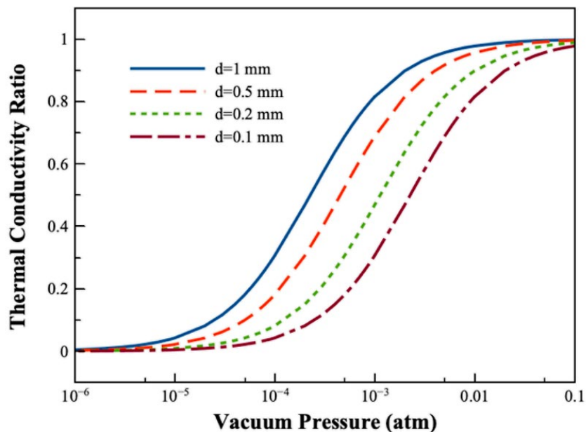
Figure 4. Thermal conductivity ratio k/k_{atm} of air versus vacuum pressure at T=300 K for various values of gap thickness.
