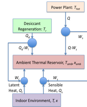
Fig. 1 Schematic diagram showing ideal system with Carnot engines and refrigerators. Note that (Q_d + Q) is the minimum primary energy input.
