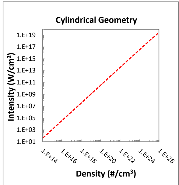
Fig. 1.b 2.b – Minimum driver intensity (W/cm 2 ) for (10 keV) D-T targets in cylindrical geometry 10
