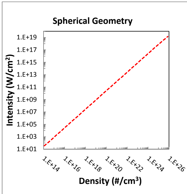
Fig. 1.a 2.a – Minimum driver intensity ( \text{W}/\text{cm}^2 ) for (10 keV) D-T targets in spherical geometry 10
