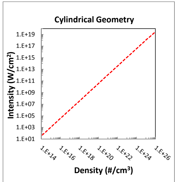
Fig. 1.b 2.b – Minimum driver intensity ( \text{W}/\text{cm}^2 ) for (10 keV) D-T targets in cylindrical geometry 10
