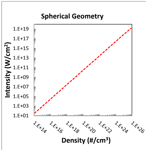
Fig. 1.a 2.a – Minimum driver intensity (W/cm 2 ) for (10 keV) D-T targets in spherical geometry 10
