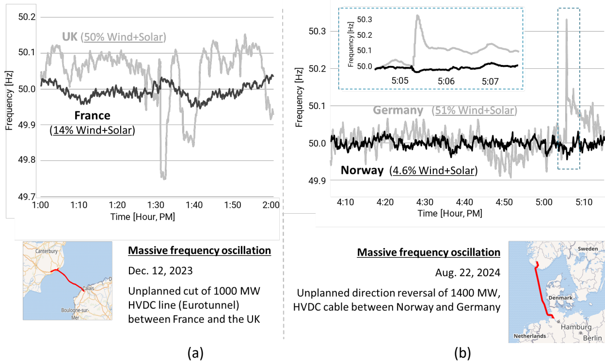
Figure 1. Electrical contingencies between (a) the United Kingdom and France and (b) Germany and Norway. 8,9 Larger frequency oscillations are observed in grids with higher IBR penetration.
