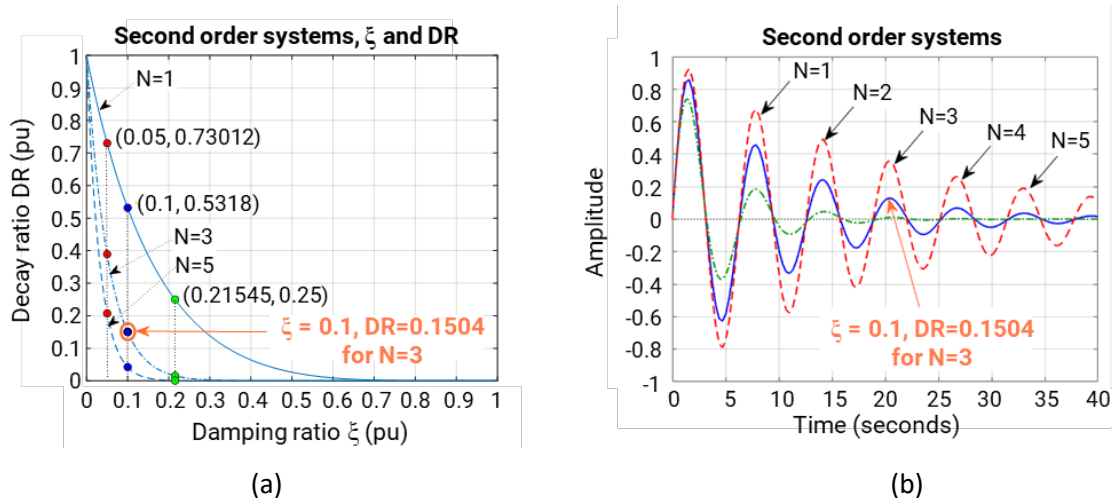
Figure 6. Simulation of a second order system, like the swing equation of a synchronous machine. (a) Representation of the relationship between damping ratio ( \xi ) and decay ratio ( DR for N ), and (b) representation of the frequency oscillation over time with three damping ratios: dashed-line \xi = 0.05 , solid-line \xi = 0.1 , dashed-dotted-line \xi = 0.21545 [or DR (for N=1 ) = 25% in Ziegler-Nichols].
