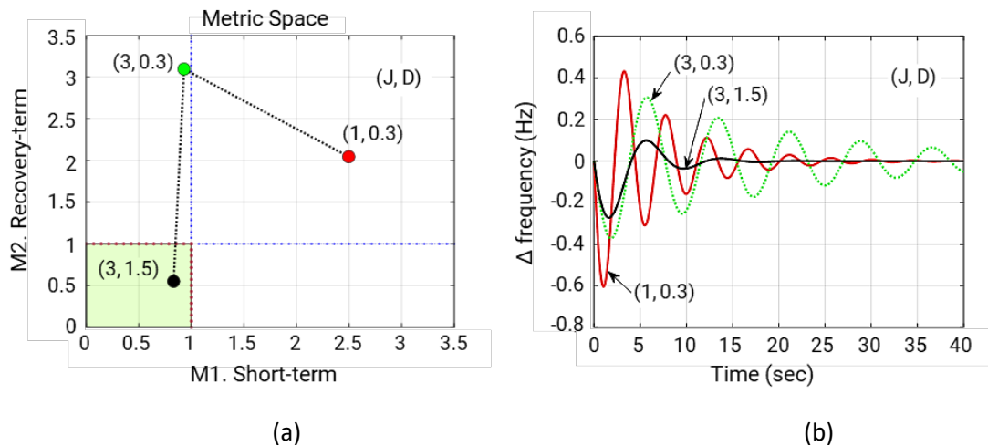
Figure 2. Results of three cases: Case 1 ( J = 1 , D = 0.3 ), Case 2 ( J = 3 , D = 0.3 ), and Case 3 ( J = 3 , D = 1.5 ). Figure (a) represents M1, or short-term metric (normalized RoCoF and nadir), versus M2, or recovery-term metric (normalized decay ratio and recovery time), and Figure (b) shows the frequency oscillation over time with these three cases.
