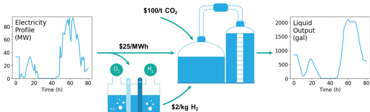
Figure 1. Black box diagram of system inputs and outputs for the reactor systems in GREENWELLS. Based on data from Iowa State University’s Automated Surface Observing System (ASOS). 7
