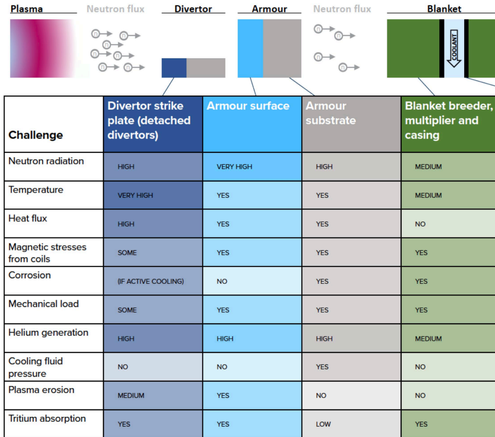
Fig. 1: Qualitative descriptions of the environments that different components of a FPP are exposed to under operating conditions 4 .
